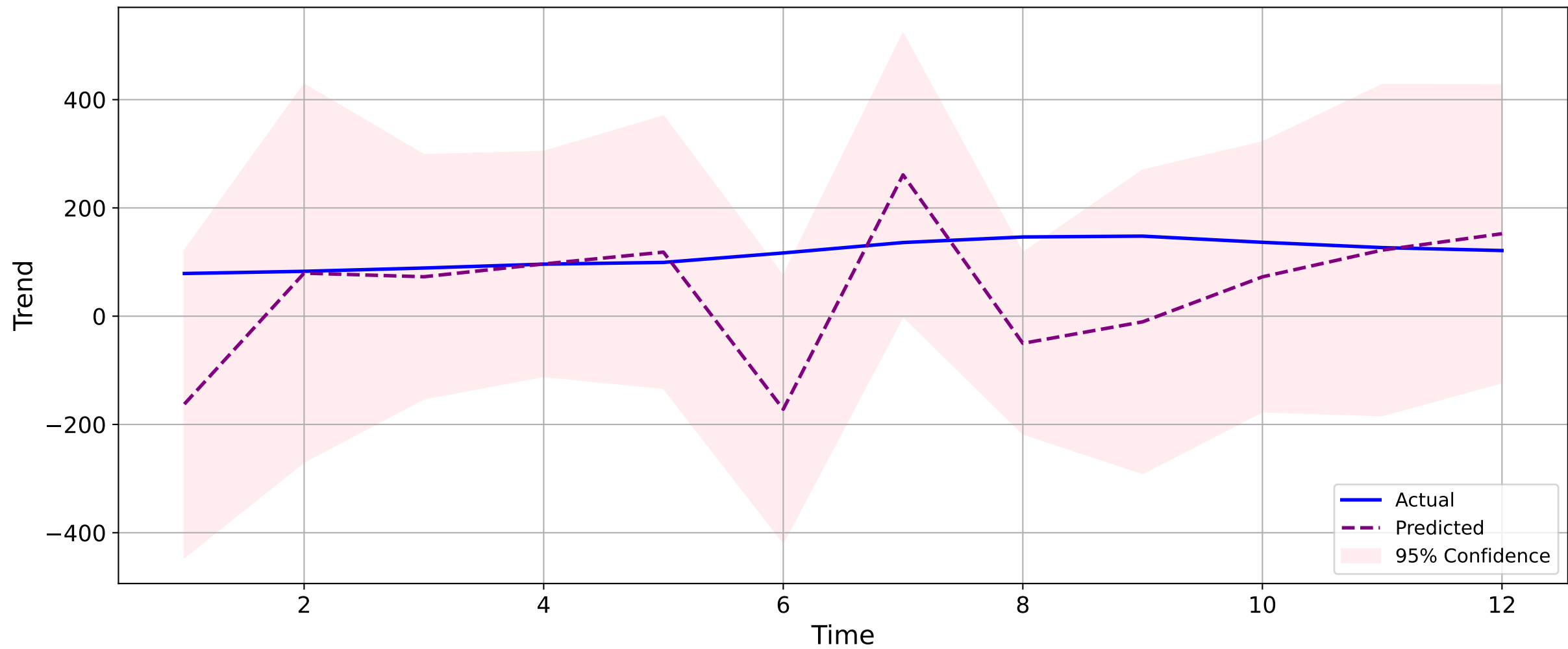
Backdoor-ALL - Validation
